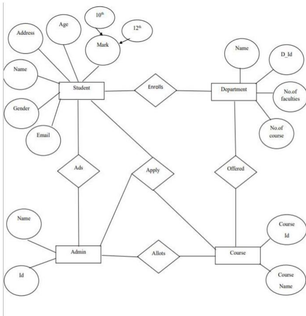
Fig: - E-R Diagram
